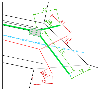
DETAIL 1 1:100
